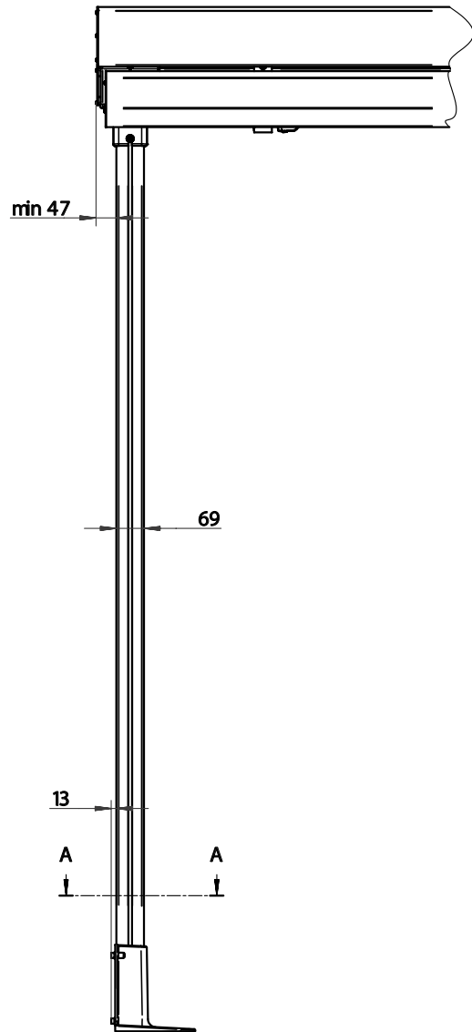
Frontvy DUO
