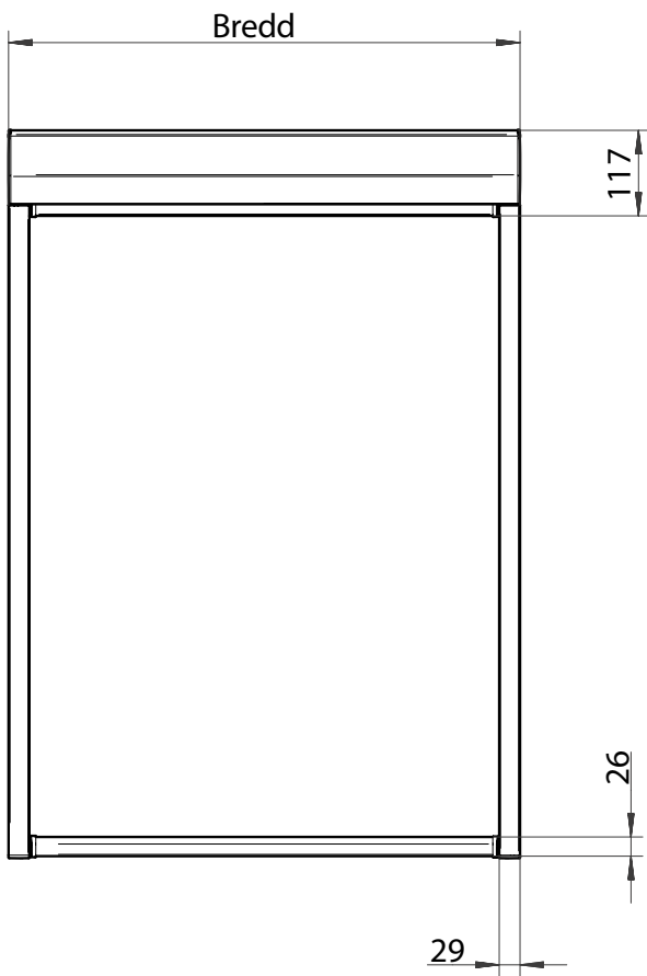
Frontvy S430
