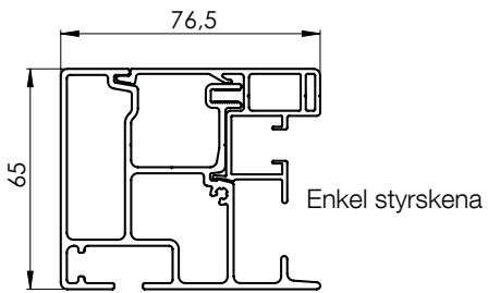
Frontvy PZ440
